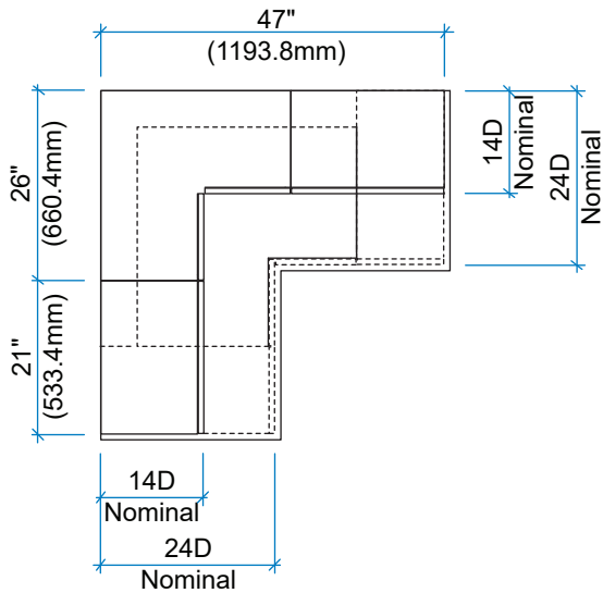
14D WALL/24D BASE L-SHAPED CORNER ALIGNMENT
