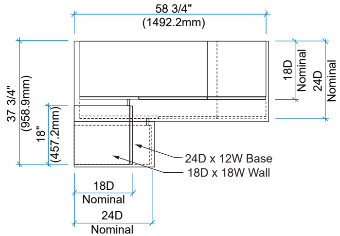
18D WALL/24D BASE BLIND CORNER ALIGNMENT
