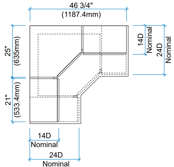
14D WALL/24D BASE DIAGONAL CORNER ALIGNMENT
