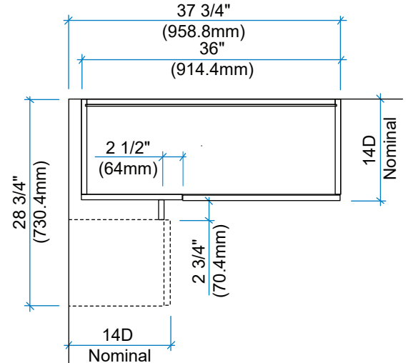
14D WALL BLIND CORNER - 36W
