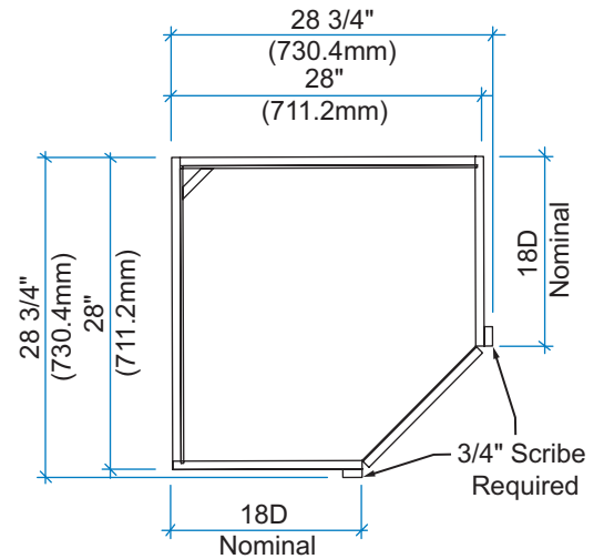
18D WALL DIAGONAL CORNER
