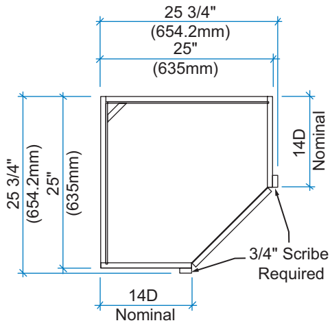
14D WALL DIAGONAL CORNER
