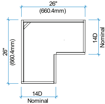
14D WALL L-SHAPED CORNER
