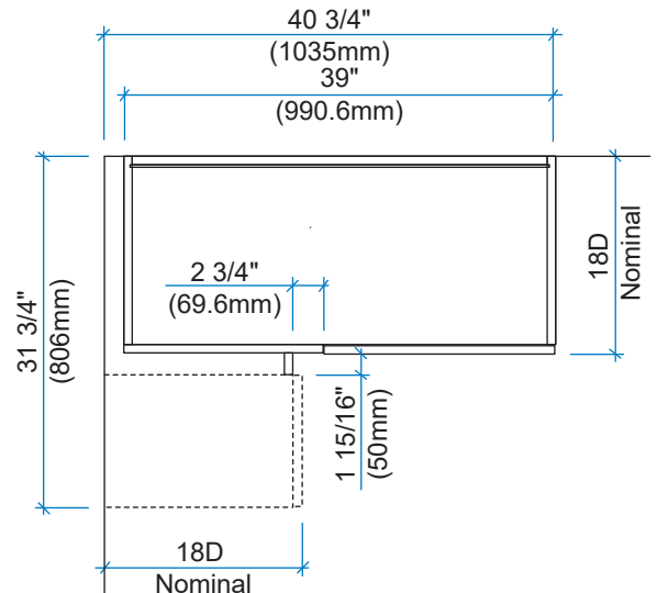
18D WALL BLIND CORNER - 39W
