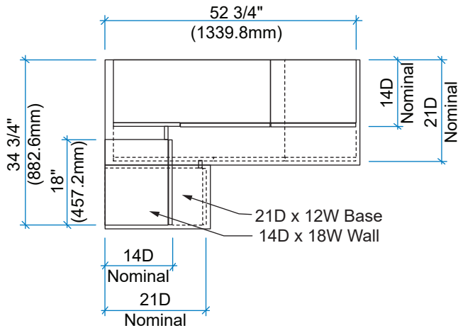
14D WALL/21D BASE BLIND CORNER ALIGNMENT
