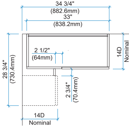
14D WALL BLIND CORNER - 33W
