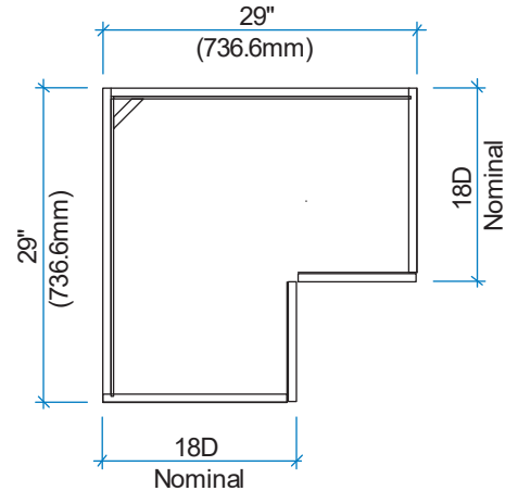
18D WALL L-SHAPED CORNER
