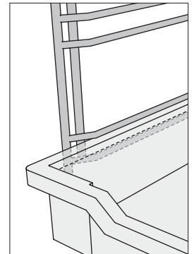
Bin and tray racks have captured runner rail to reduce tray tipout.
