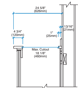
NOMINAL 24 SLIDING DOOR SINK CABINET DEPTH
