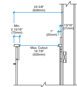
NOMINAL 24 SINK CABINET DEPTH
