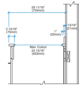
NOMINAL 29 SINK CABINET DEPTH
