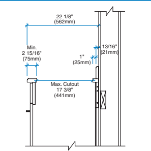
NOMINAL 21 SINK CABINET DEPTH
